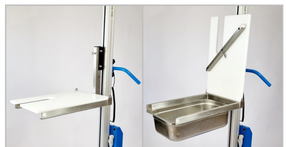
Art 75000K. GN 1/1 fork foldable platform milk box 575x380x57 mm.
